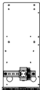
1031,5077 Montageplatte komplett mounting plate complete plaque support de commande
