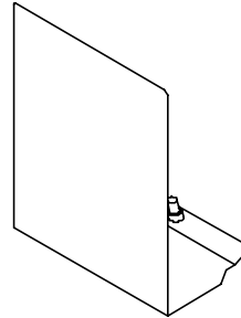
2067,5009 Alu-Frontplatte aluminium front plate face avant aluminium
